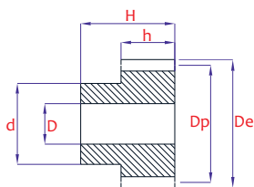
Modul 3; h=30mm; H=50mm
