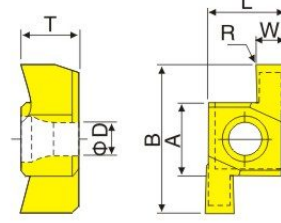
图B 双头 Fig. B Double-head
